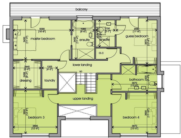
first floor plan (upper & lower)
